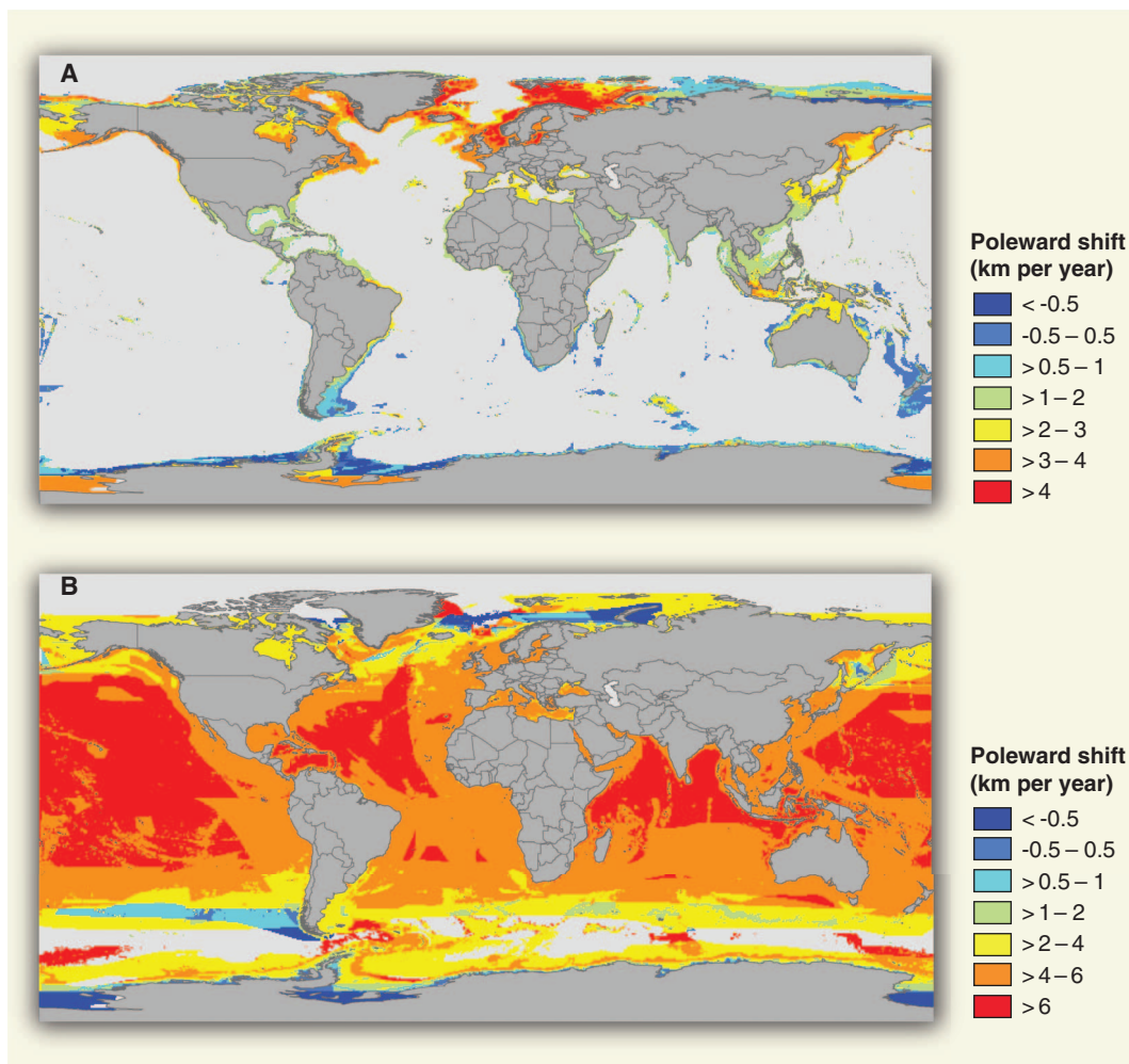
Fig. 4. Projected rate of range shifts in marine organisms caused by climate change from 2005 to 2050 (52, 63). (A) Latitudinal shift of demersal species (excluding areas >2000 \text{ m} in depth because of undersampling of the deep-sea region). (B) Latitudinal shift of pelagic species. The projections are based on bioclimatic envelope models for 1066 species of fish and invertebrates, under IPCC SRES A1B. For each map cell, the mean shift of the range centroids of the species currently present in that cell is given.
